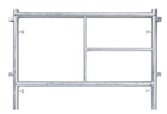
梯型门架 Φ42.5*2.4mm
