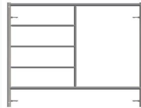
梯型门架 Φ42.5*2.4mm
